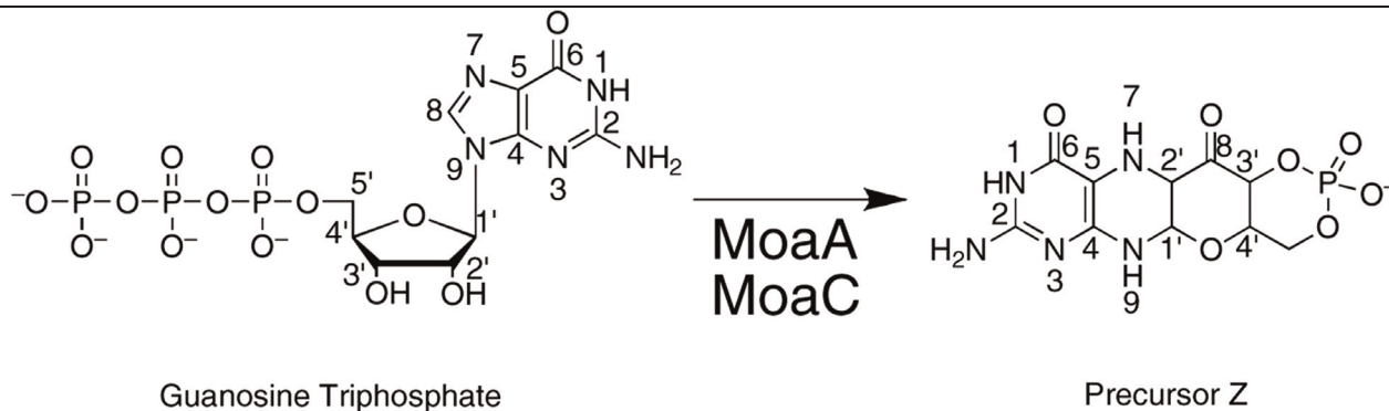
Figure 4. The reaction catalyzed by MoaA/MoaC
