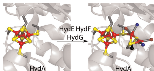
Figure 2. Maturation of the H-cluster of the [FeFe]-hydrogenase
