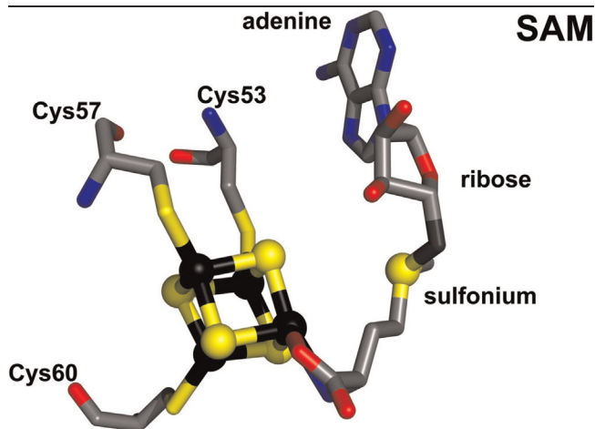
Figure 1. Binding mode of SAM in radical SAM proteins
