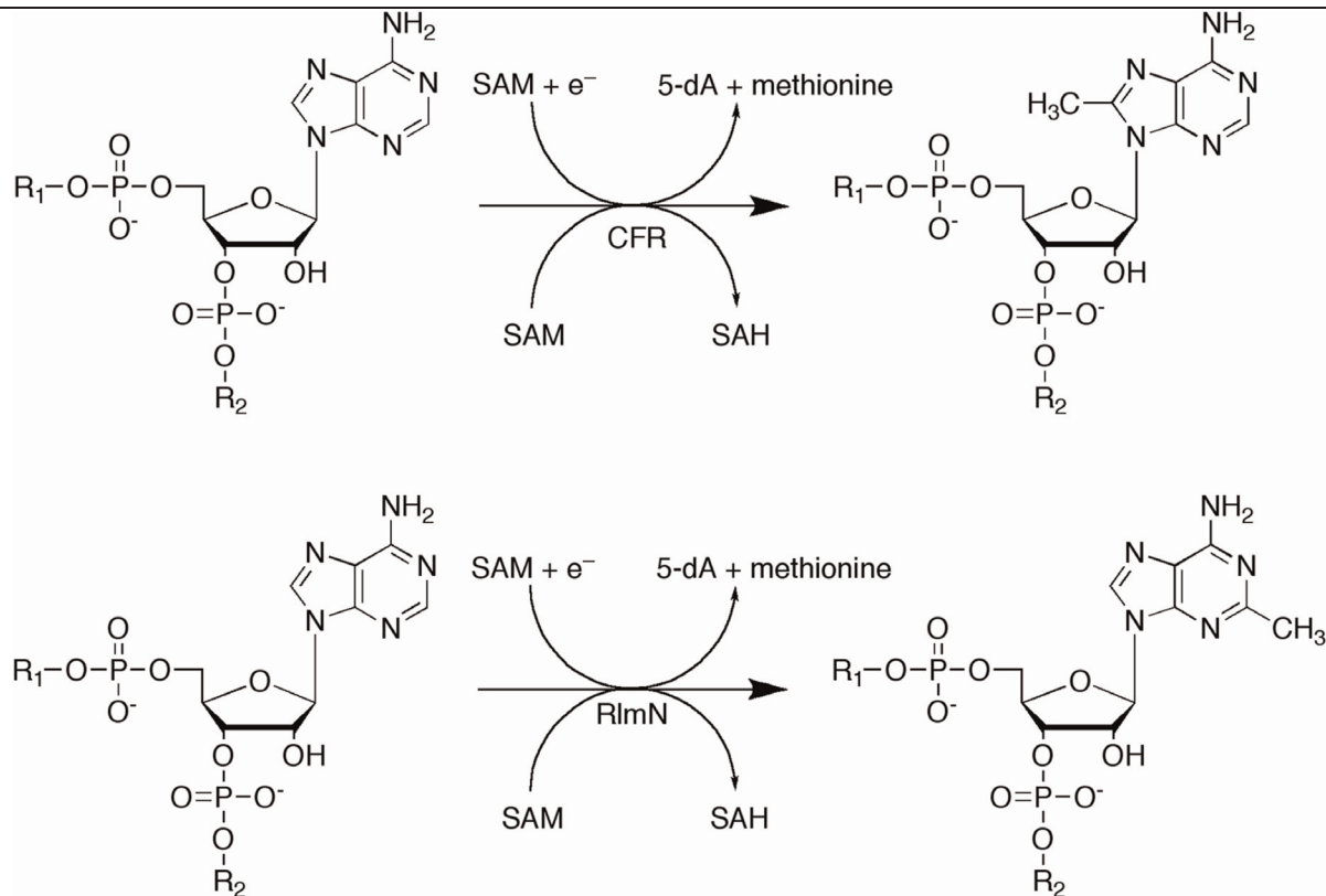
Figure 6. The reactions catalyzed by Cfr and RlmN
