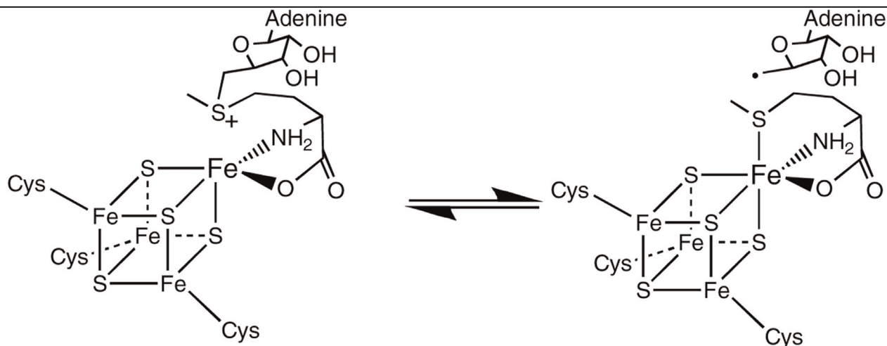
Figure 7. Model for the reductive cleavage of SAM to generate a 5'-deoxyadenosyl radical
