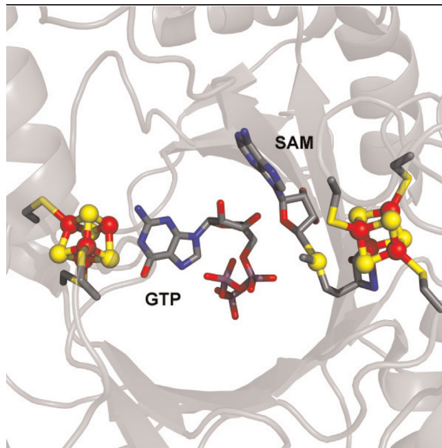
Figure 5. The active site of MoaA
