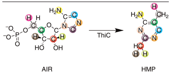
Figure 3. The reaction catalyzed by ThiC
